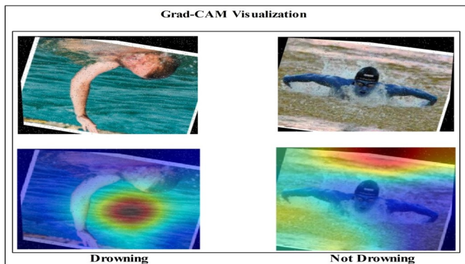
Figure 8: Grad-CAM visualization of the proposed drowning detection framework.
