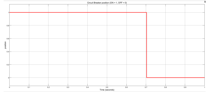
Figure 12: Breaker position under DLG fault.
