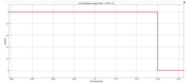
Figure 7: Circuit breaker trip control showing 3 ms delay.
