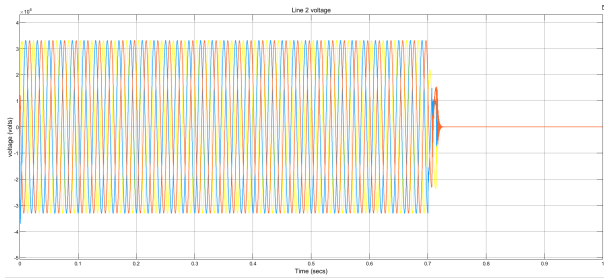
Figure 4: Line-2 voltage under 3-LG fault.
