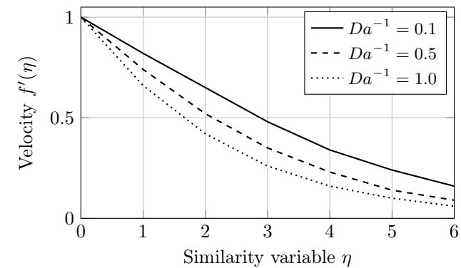
Figure 2: Velocity profiles for varying inverse Darcy number.
