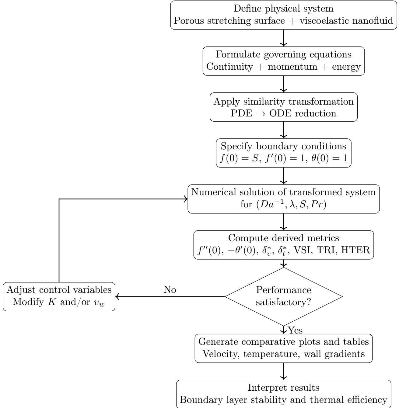
Figure 1: Methodological workflow for inverse Darcy-driven nanofluid flow regulation over porous stretching surfaces.
