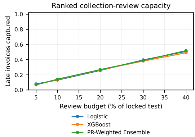
Figure 8: Surrogate late-invoice retrieval under fixed review budgets.
