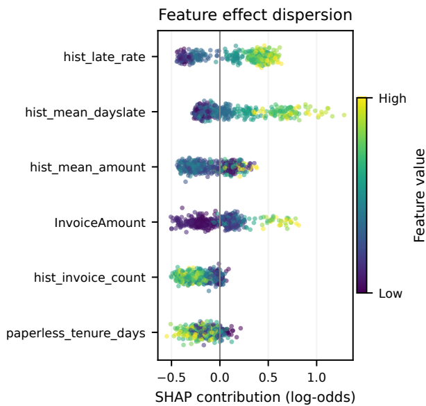
Figure 7: Surrogate SHAP contribution dispersion for the six strongest transformed features.
