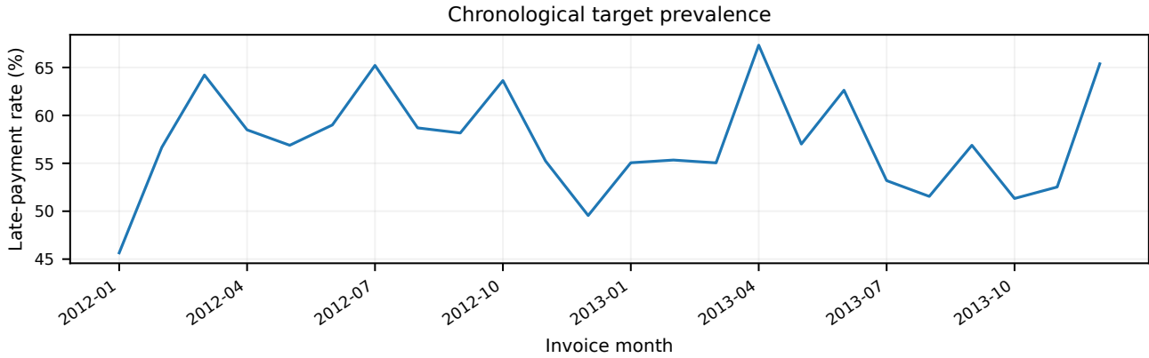
Figure 2: Chronological target prevalence in the deterministic pipeline-verification surrogate.
