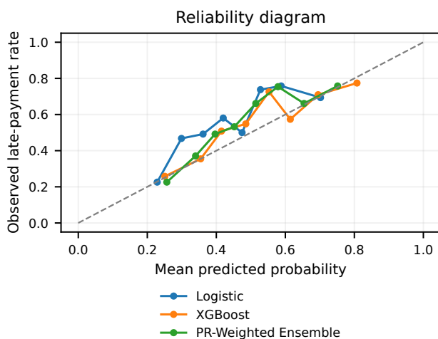
Figure 5: Surrogate reliability diagram.
