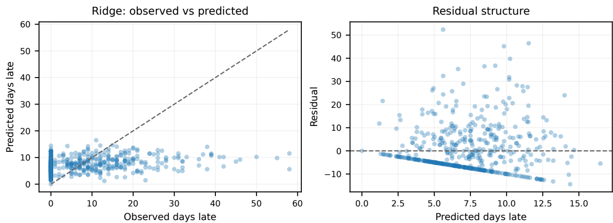
Figure 4: Surrogate pipeline-verification regression diagnostics for the lowest-RMSE model.
