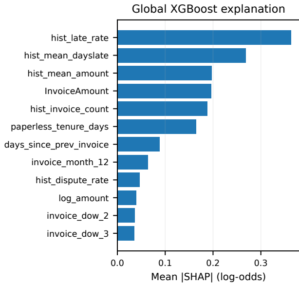
Figure 6: Global mean absolute TreeSHAP values in the deterministic surrogate verification run.
