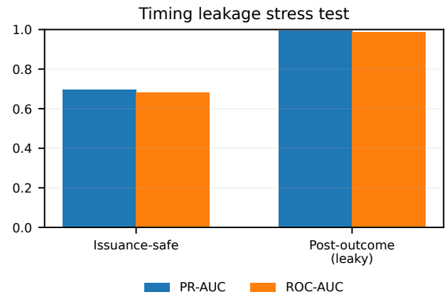
Figure 9: Deliberate timing-leakage stress test on the surrogate.
