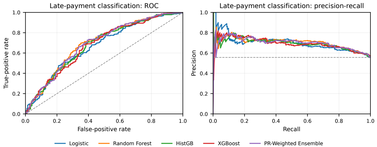
Figure 3: Surrogate pipeline-verification ROC and precision–recall curves.
