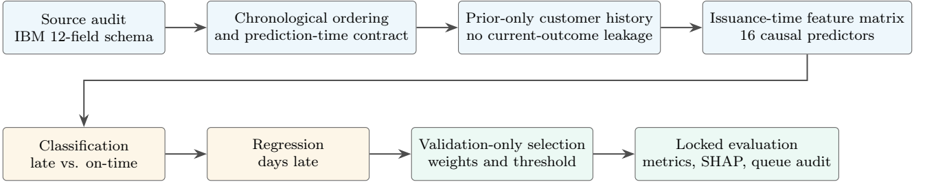
Figure 1: End-to-end experimental workflow.
