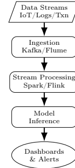
Figure 6: Low-latency pipeline for real-time analytics and alerting.
