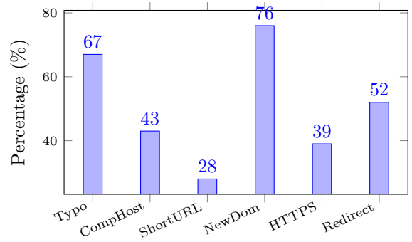
Figure 10: URL-based phishing indicators.
