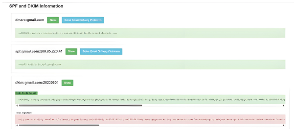
Figure 7: DKIM and domain key verification.
