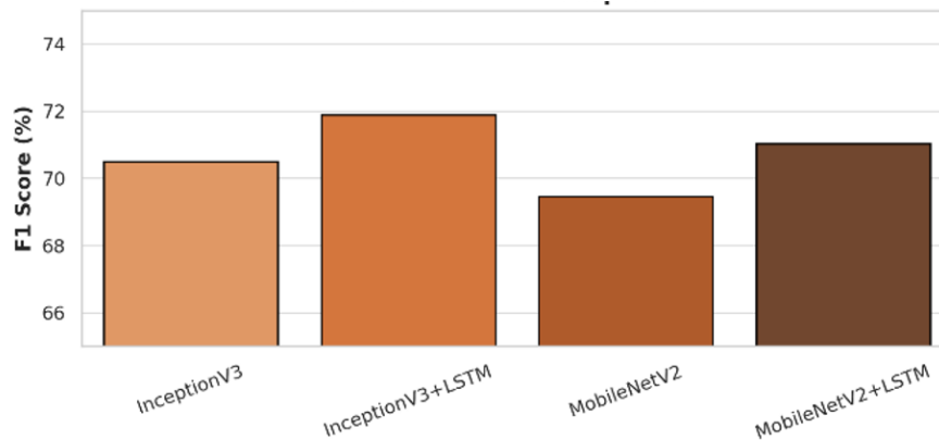
Figure 6: Classification accuracy of the evaluated models.
