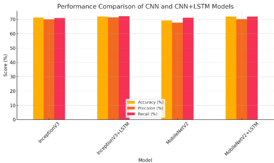
Figure 2: Accuracy, precision, and recall comparison of the models considered in the proposed study.
