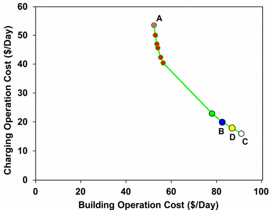
Figure 1: Pareto frontier analysis of building and charging station integration operational costs.
