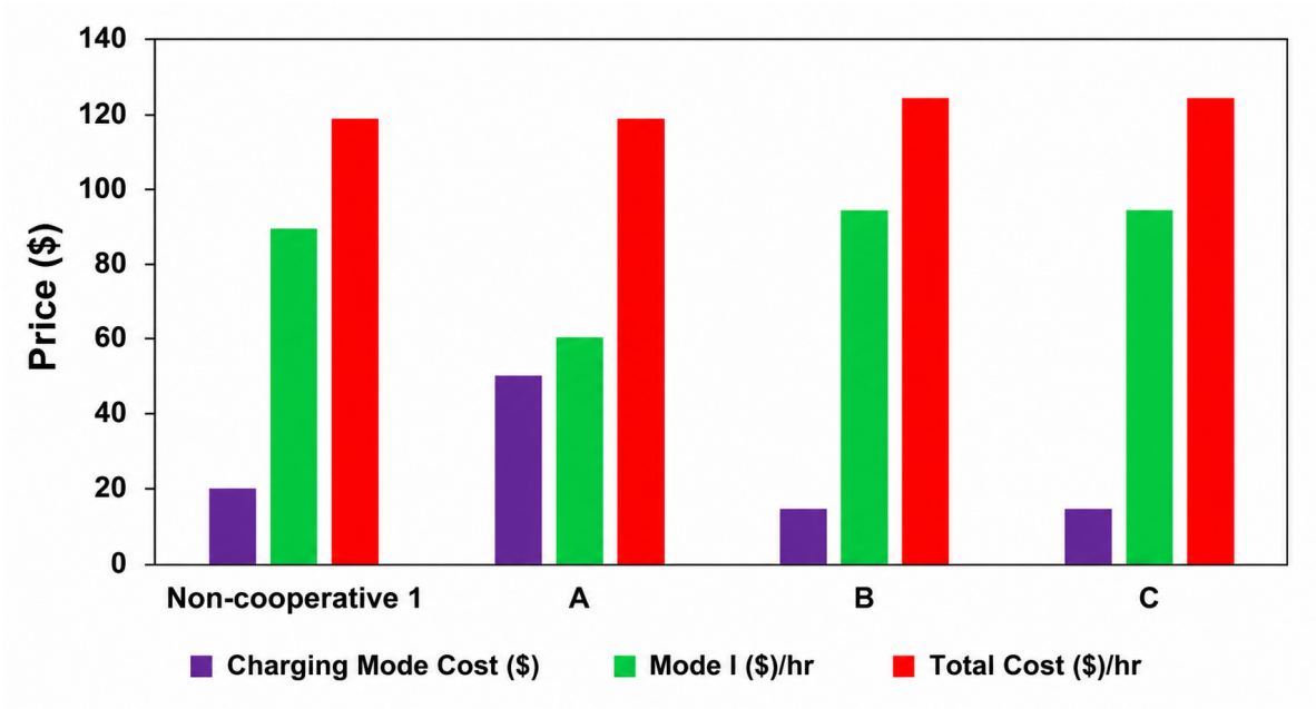
Figure 4: Comparing operational strategies: collaborative and non-cooperative.
