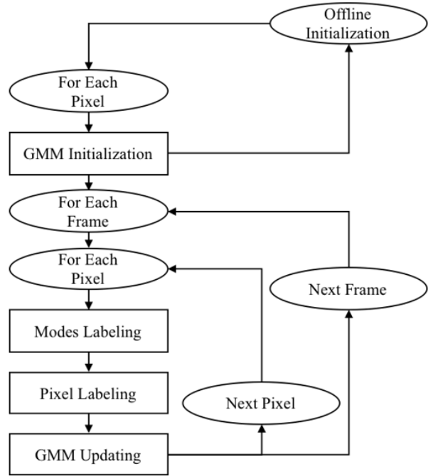
Figure 4: Adaptive Gaussian Mixture Model (GMM) for background and foreground separation.
