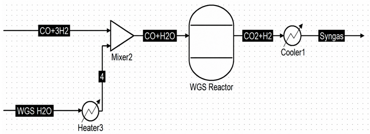
Figure 2: Water-Gas Shift (WGS) reaction simulation.
