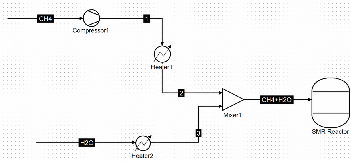
Figure 1: Steam methane reforming simulation.
