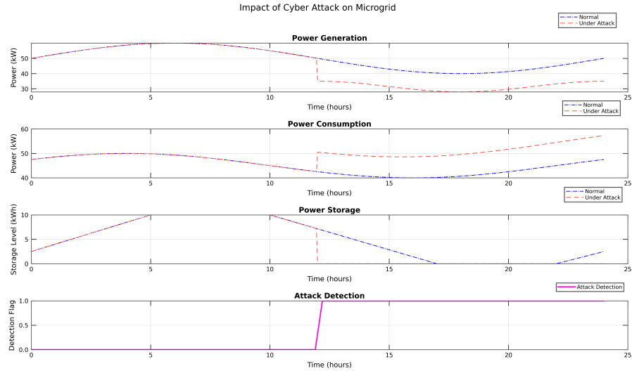
Figure 4: Power generation, power consumption, and power storage under normal, and attack situation including the primary attack detection.
