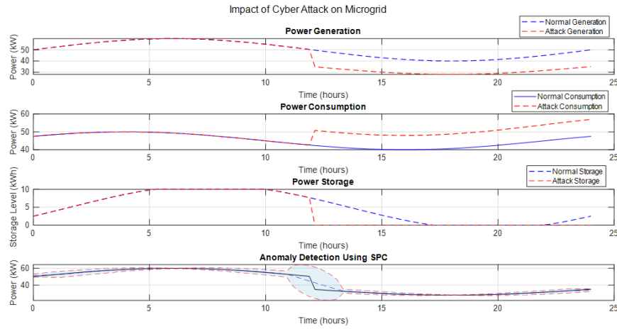
Figure 5: Applying enhanced detection approach based on SPC.
