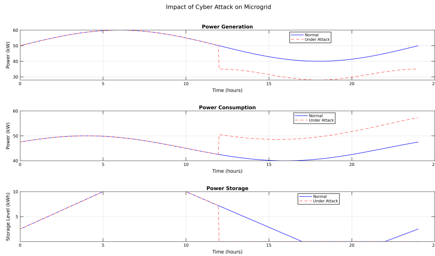
Figure 3: Power generation, power consumption, and power storage under normal, and attack situation.
