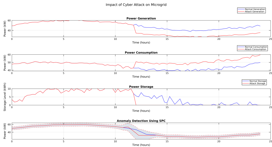
Figure 6: Applying enhanced detection approach based on SPC.
