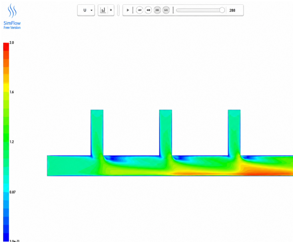
Figure 10: Velocity profile of flow.
