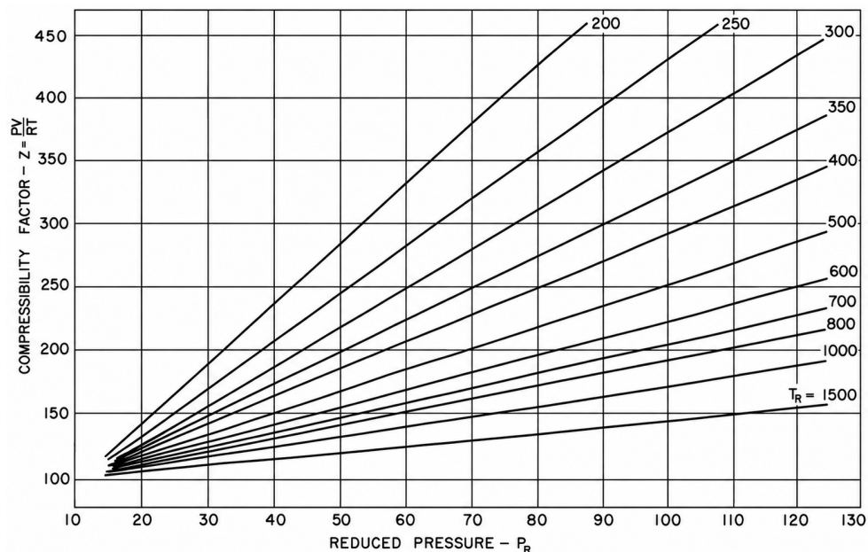
Figure 2: Hydrogen compressibility chart - high pressure range [10].
