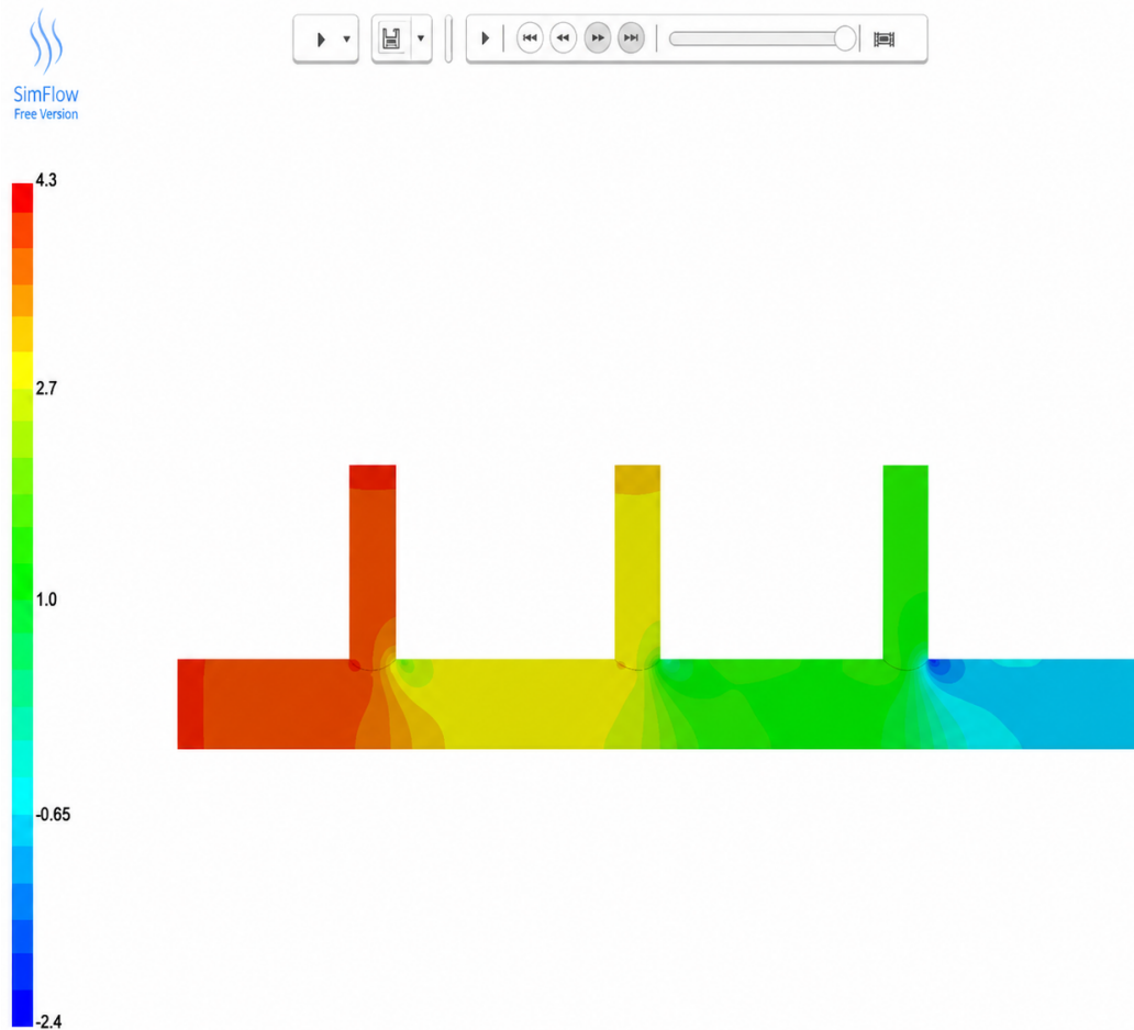
Figure 11: Pressure profile of flow.
