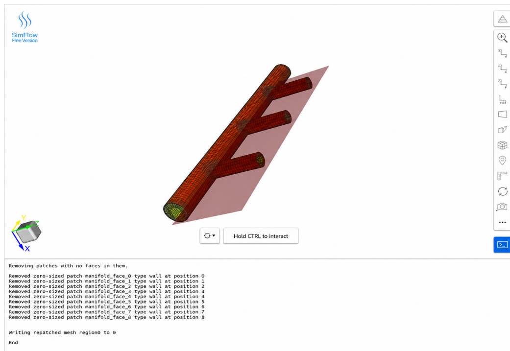
Figure 5: Meshed geometry (Face groups in green).
