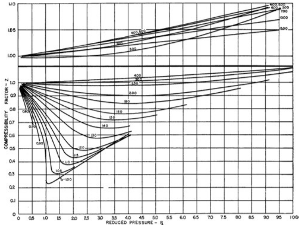
Figure 1: Hydrogen compressibility chart - low pressure range [9].
