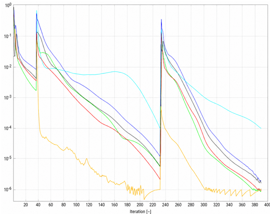
Figure 12: Residual convergence for hydrogen flow in pipeline manifold.
