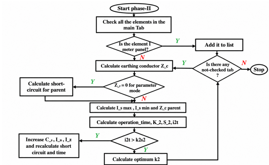
Figure 3: Cable sizing algorithm and influence of short circuit.
