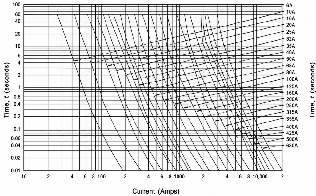
Figure 4: Relation between Time-Current for fuse selection.
