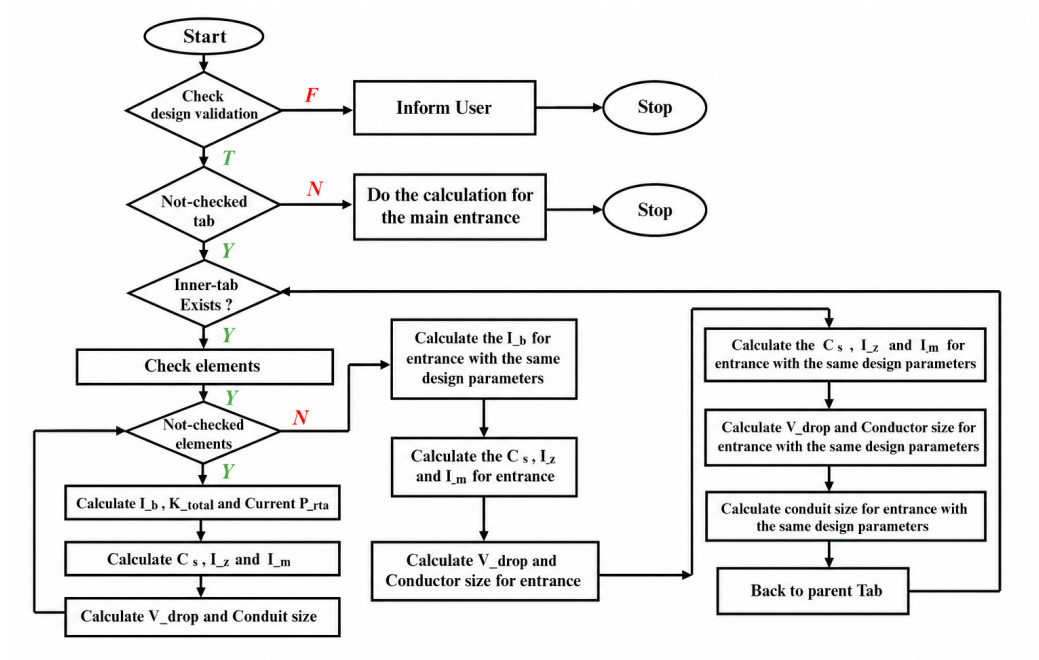
Figure 2: Algorithm for sizing cable.
