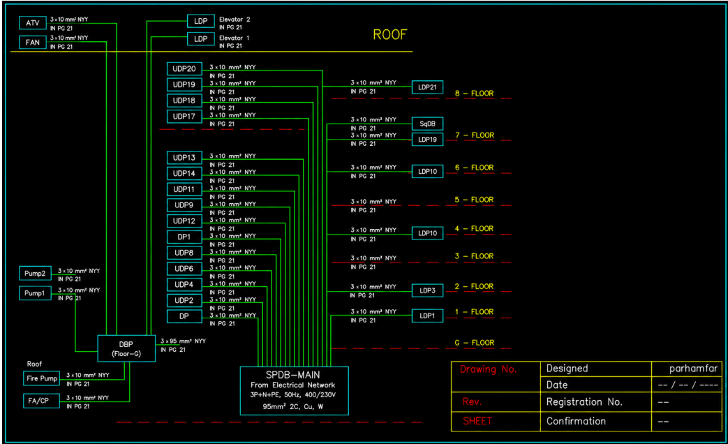
Figure 7: Sample of riser diagram exported in AutoCAD.
