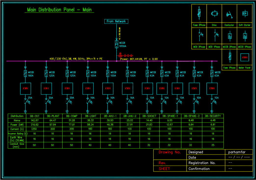
Figure 6: Sample of a single diagram exported in AutoCAD.
