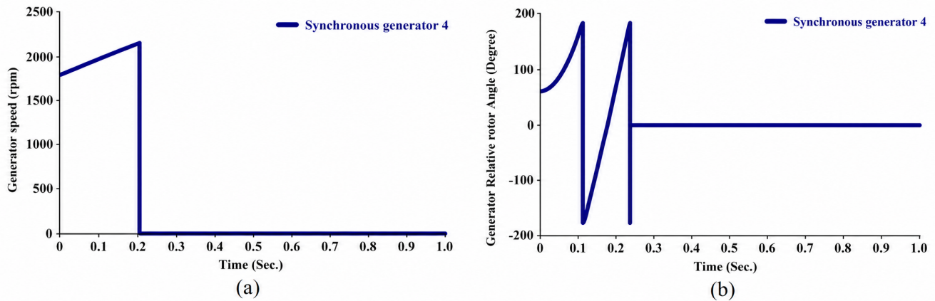
Figure 10: Transient stability emulation of synchronous generator 4, (a) generator speed (RPM), (b) synchronous generator power angle (degrees).
