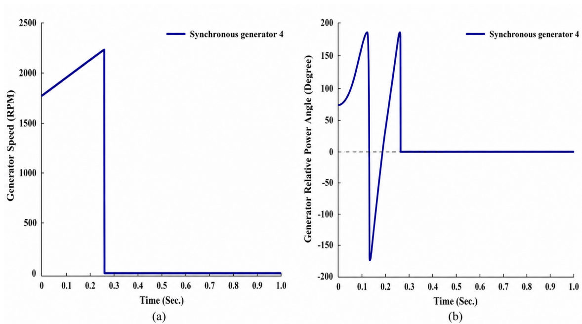
Figure 9: Transient stability emulation of synchronous generator 3, (a) generator speed (RPM), (b) synchronous generator power angle (degrees).
