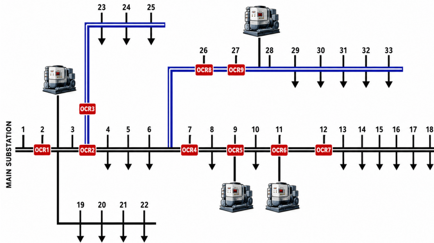
Figure 2: Protection-oriented one-line schematic of the analyzed network [28].
