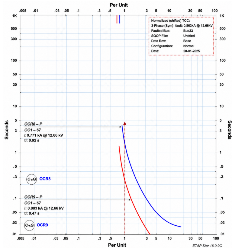
Figure 13: Coordination between OCRs in scenario 5 for Bus 33.
