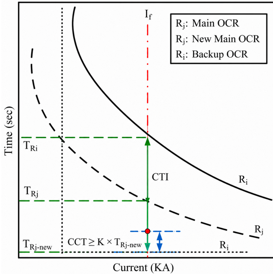
Figure 6: Modify the primary relay curve.
