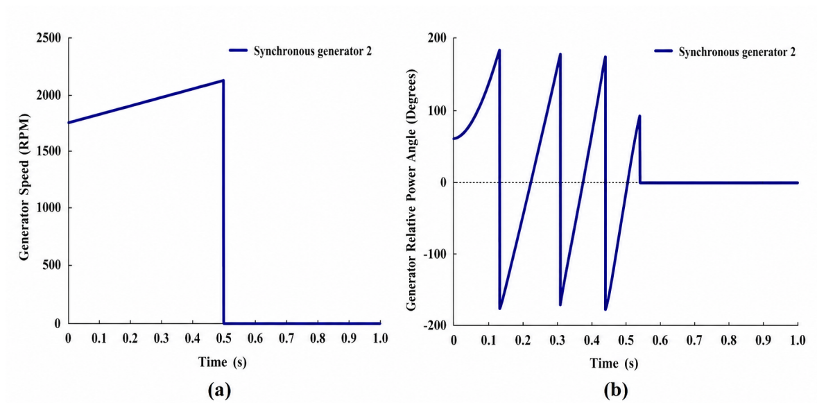
Figure 8: Transient stability emulation of synchronous generator 2, (a) generator speed (RPM), (b) synchronous generator power angle (degrees).
