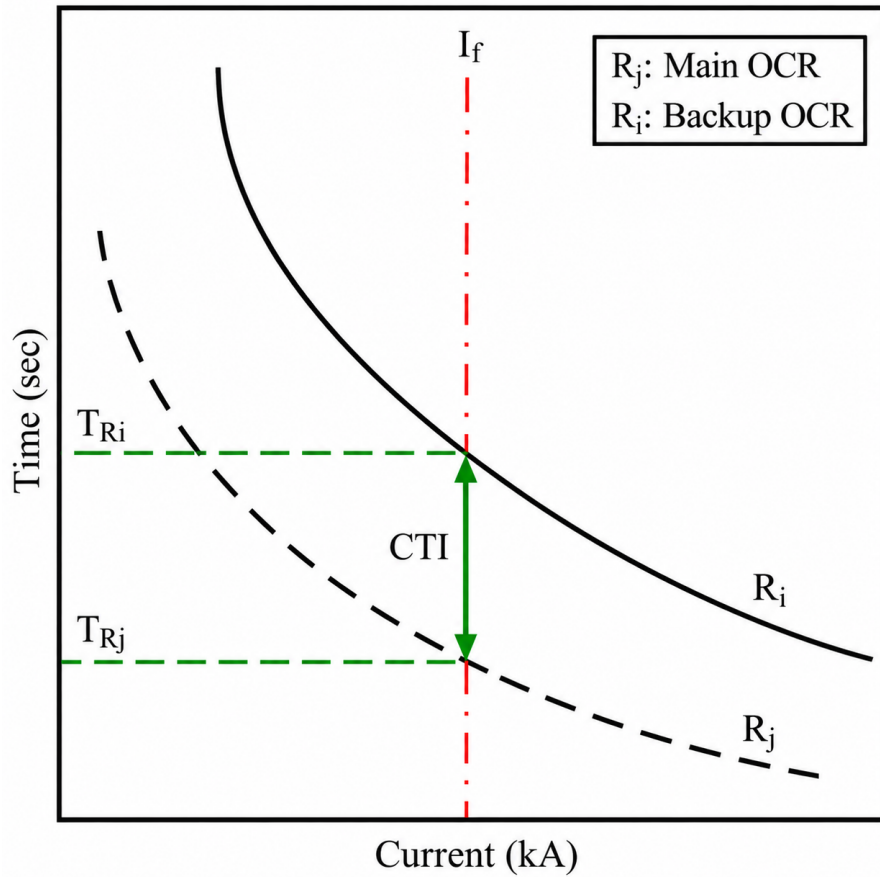
Figure 5: Establishing the CTI constraint between OCRs.
