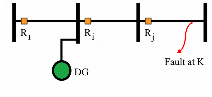
Figure 4: A typical power system includes DG sources with overcurrent protection.
