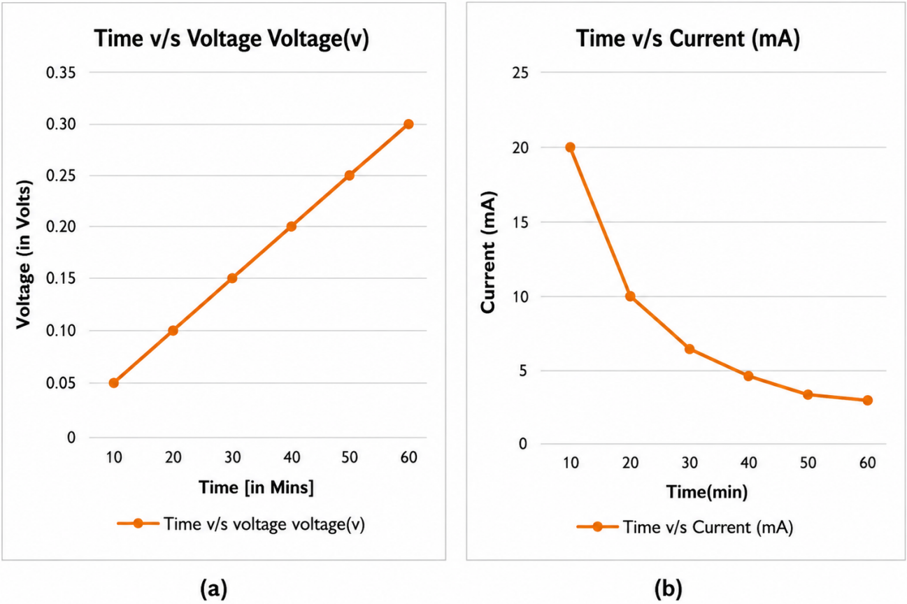
Figure 13: Charging over time (a): voltage, (b): Current charging over time.
