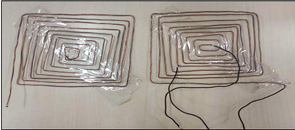
Figure 5: Square spiral coil of 10 turns with thickness of 2mm with 1mm gap.
