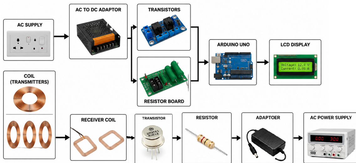
Figure 4: Block diagram of dynamic WPT.
