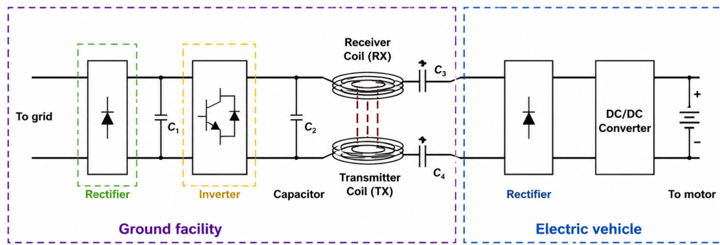
Figure 3: Typical WPT charging system for electric vehicle.
