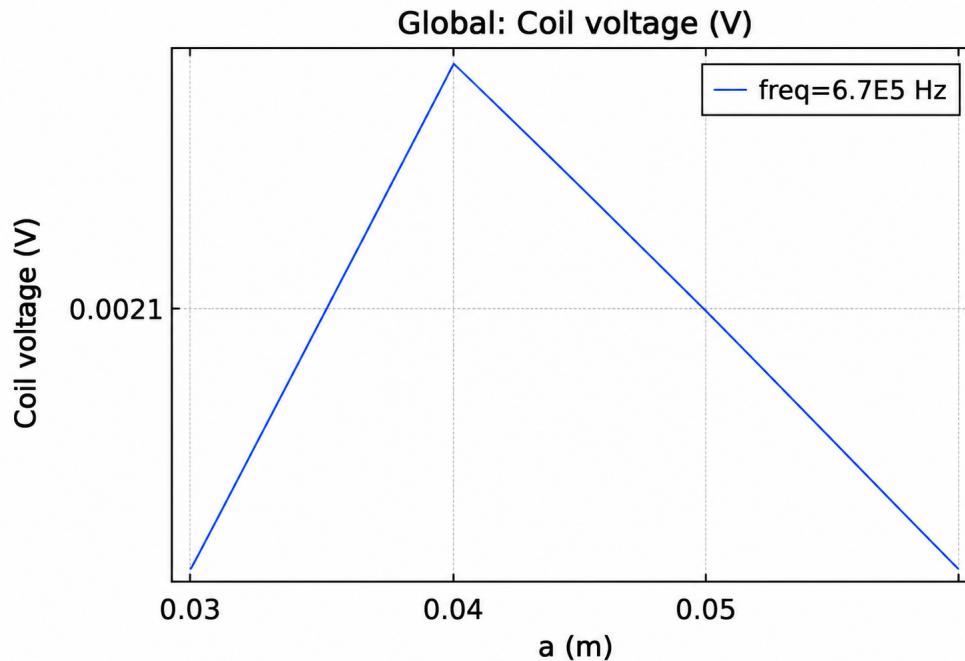
Figure 16: Voltage observed at receiver coils.
