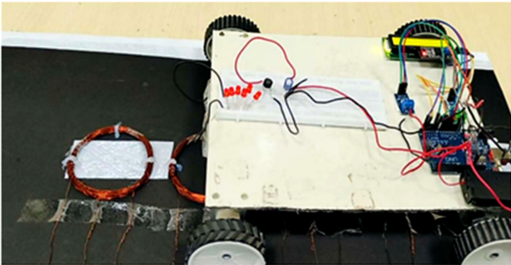
Figure 9: Experimental setup of dynamic WPT.
