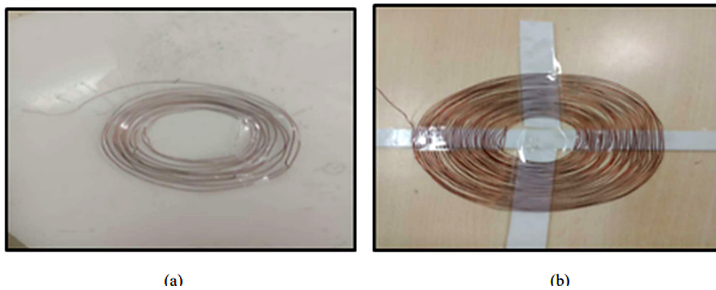
Figure 6: Circular Spiral Coil (a): 10 turns, (b): 30 turns.
