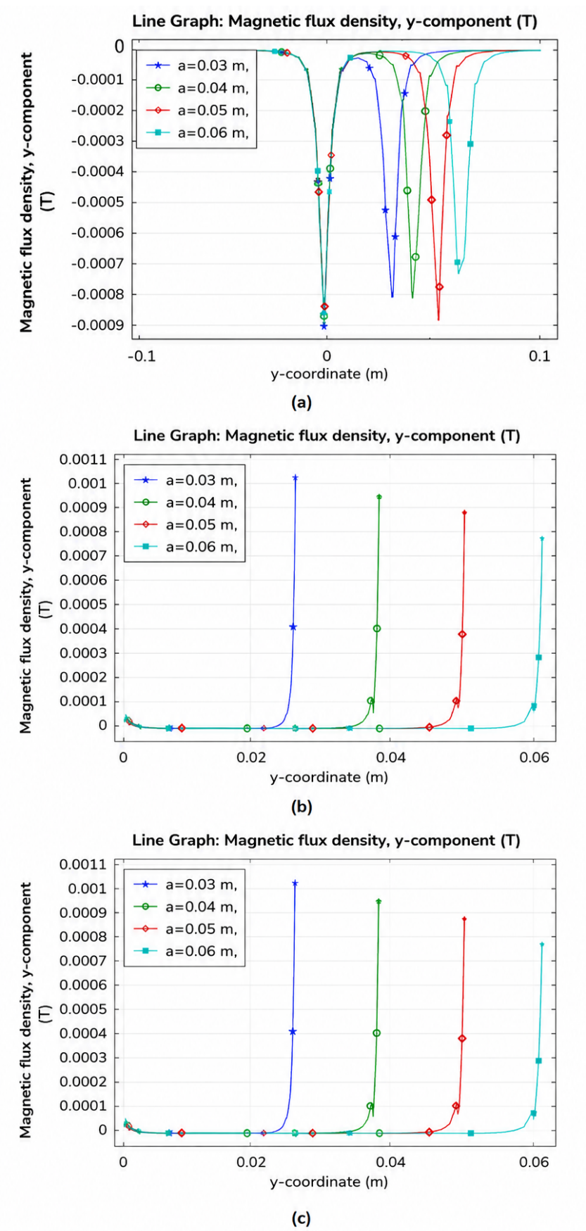
Figure 15: Magnetic flux distribution between (a): Middle of transmitter and receiver (b): Left transmitter to middle transmitter (c): Right transmitter to middle transmitter.
