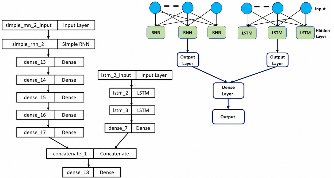
Figure 4: Proposed hybrid RNN-GRU-LSTM architecture.
