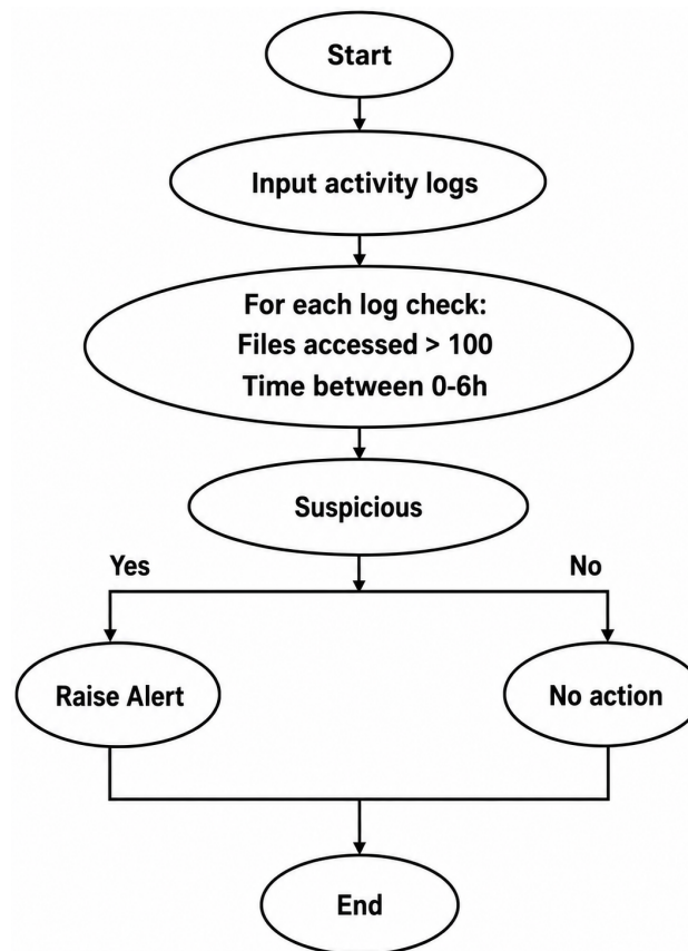
Figure 2: Scanning the sensitive data (section 1.2).
