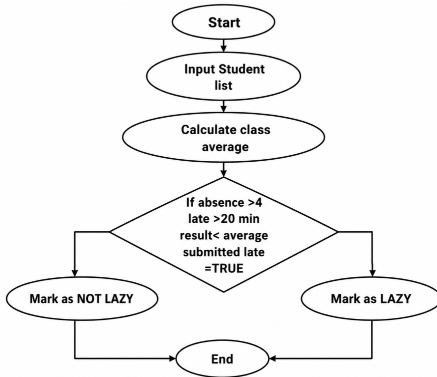
Figure 7: Flow of execution of the code.
